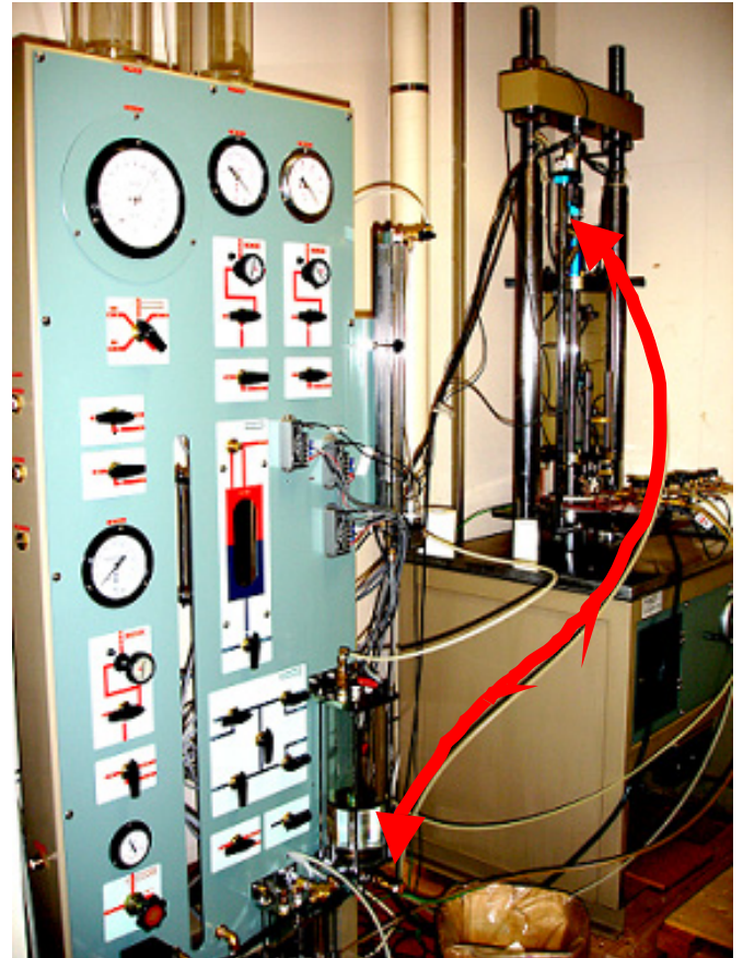
Fig 1.4 The new triaxial apparatus
