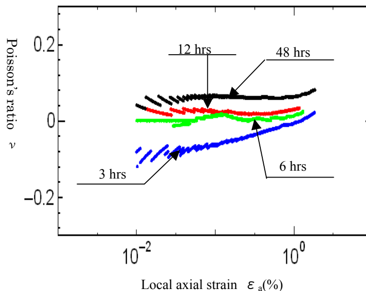
Fig 3.3 Relationships between axial strain \epsilon_a and Poisson's ratio \nu
