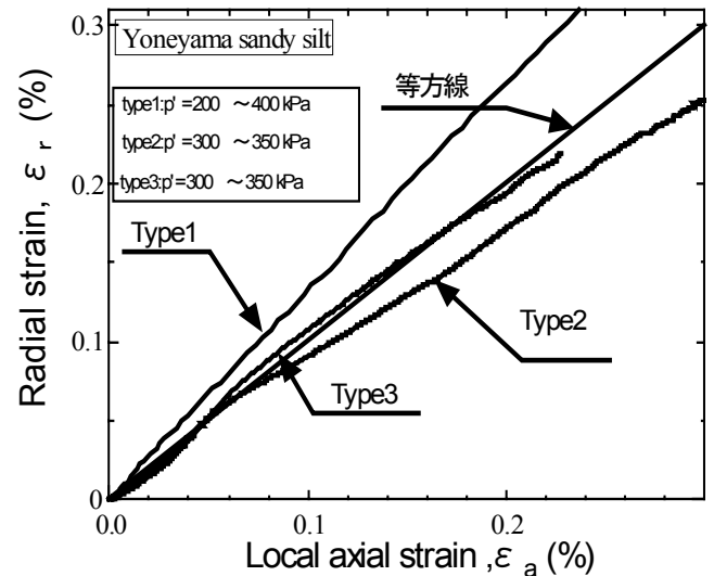
Fig 3.1 Relationships between axial strain and radial strain during saturated isotropic consolidation
