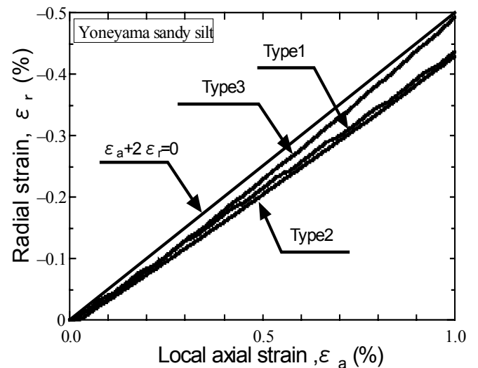
Fig 3.2 Relationships between axial strain and radial strain during consolidated-undrained shearing test
